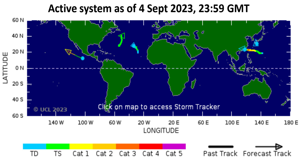
Figure 3. A tropical depression risk observed on 04 Sept 2023.
