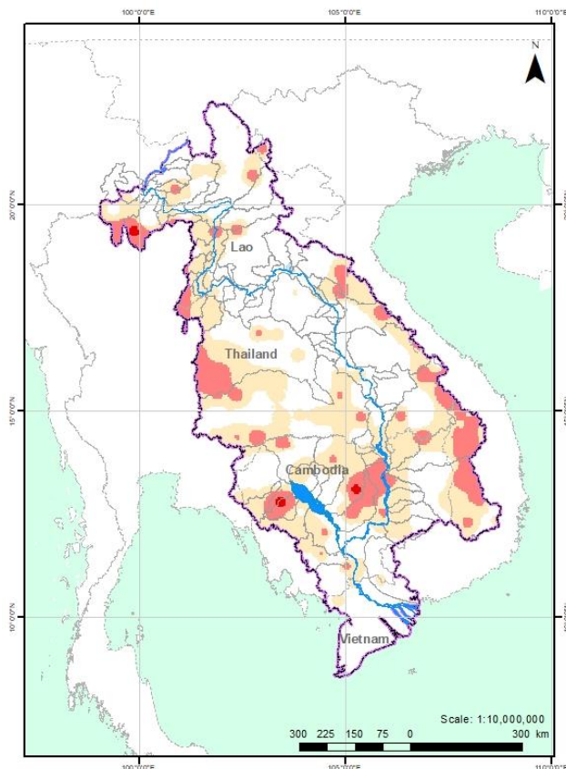
Figure 15. Weekly standardized precipitation index from 28 August to 3 September 2023.
