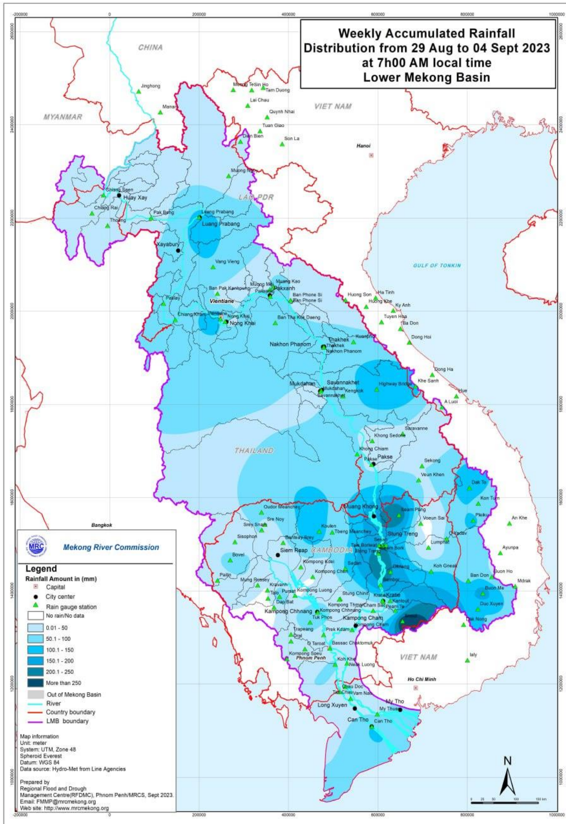
Figure 5. Weekly rainfall distribution over the LMB during 29 Aug-04 Sep 2023.
