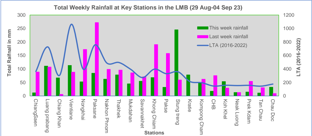
Figure 4. Weekly total rainfall at key stations in the LMB during 29 Aug-04 Sep 2023.
