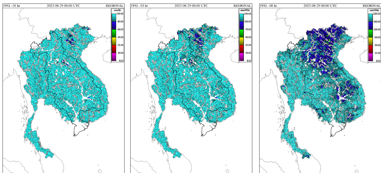
Figure 14. Flash Flood Guidance for the next 1-hr, 3-hr and 6-hr on August 29
