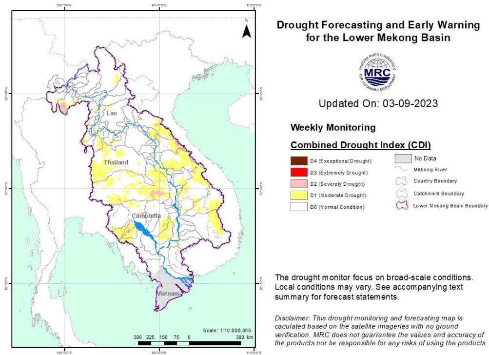
Figure 17. Weekly Combined Drought Index from 28 August to 3 September 2023.
