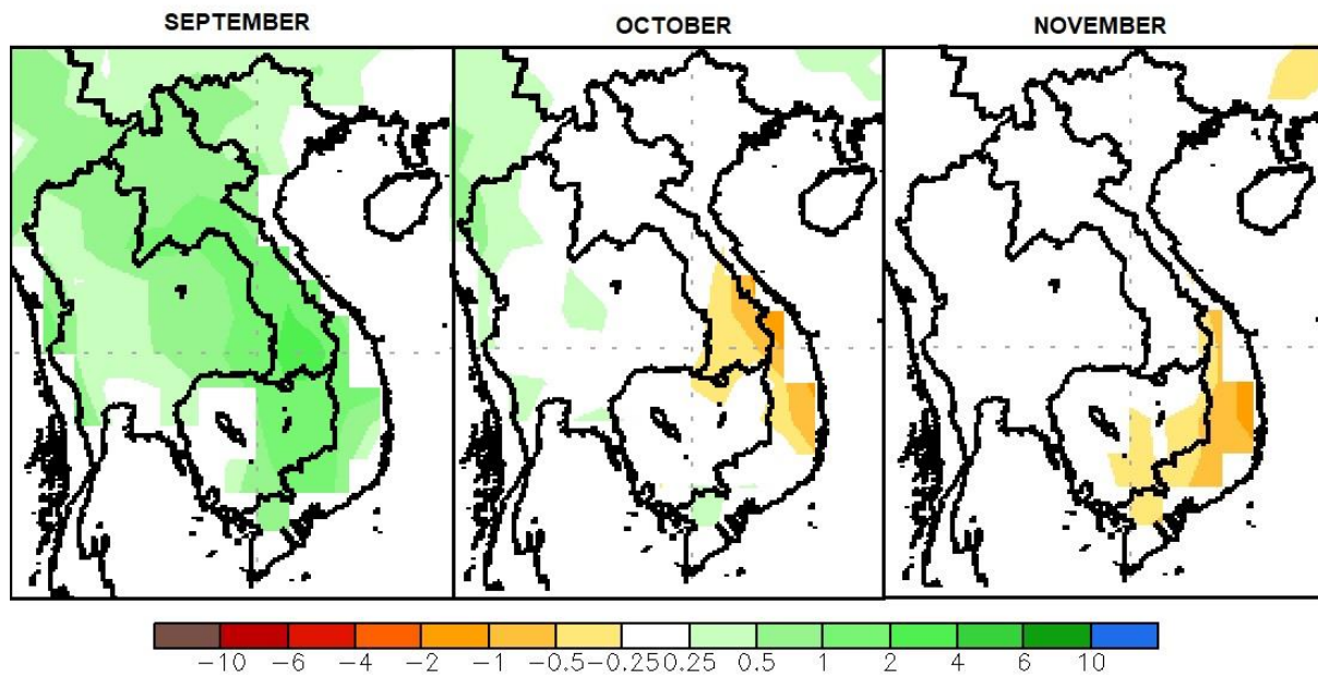
Figure 19. Monthly forecasts of precipitation anomaly in millimeters for September, October, and November 2023.
