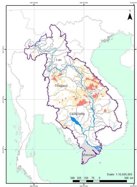
Figure 16. Index of Soil Water Fraction from 28 August to 3 September 2023.
